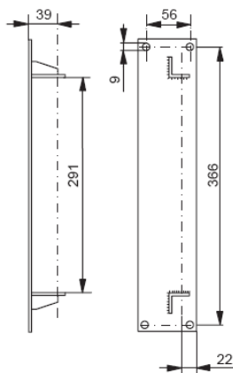
Support mural
